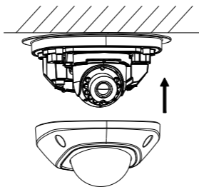
Figure 2-6 Install the Front Cover
