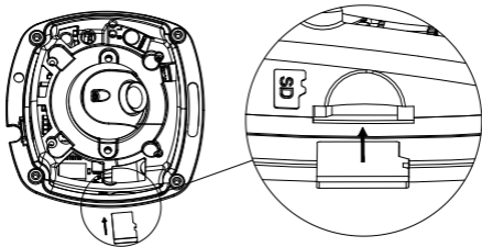
Figure 2-21 Install Micro SD Card
