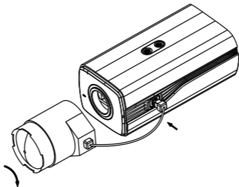
Figure 2-1 Fix the Camera on the Back-plane
