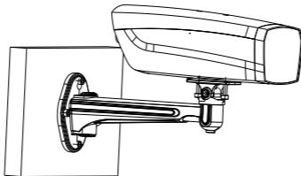
Figure 2-6 Fix the Camera Housing
