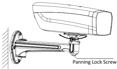
Figure 2-7 Adjust the Panning Angle
