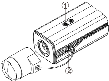
Figure 1-1 Overview of the Box Camera
