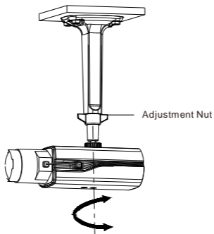
Figure 2-12 Angle Adjustment
