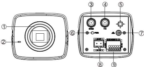
Figure 1-3 Panel Description of the Box Camera
