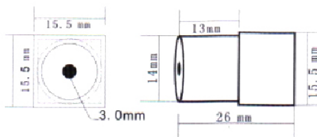
MC91AB18 Outline Size
